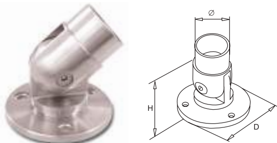
ARTICULATED WALL PLATE
