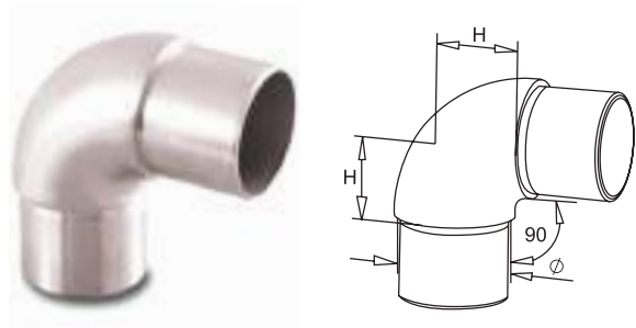
90° CURVED ELBOW
