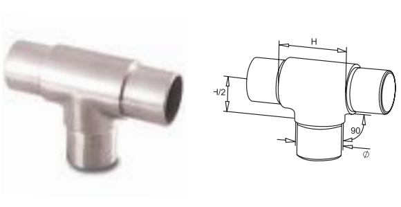
EQUAL TEE
