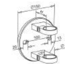
ROUND POST HOLDER
