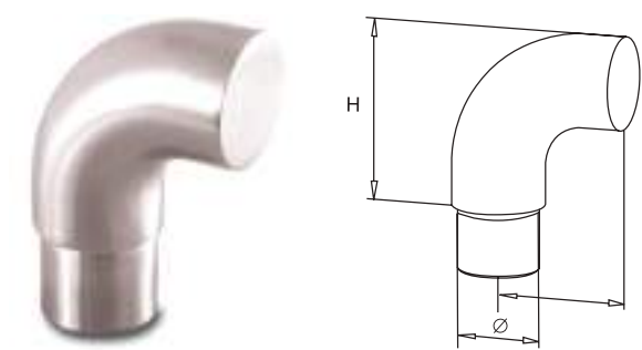
90° CURVED ELBOW M/F (with Cap)
