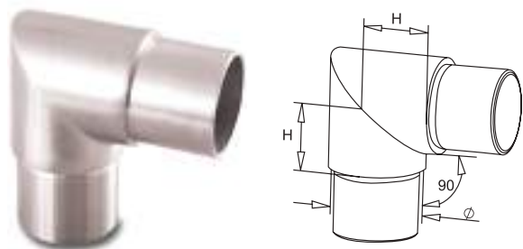
90° SHARP ELBOW
